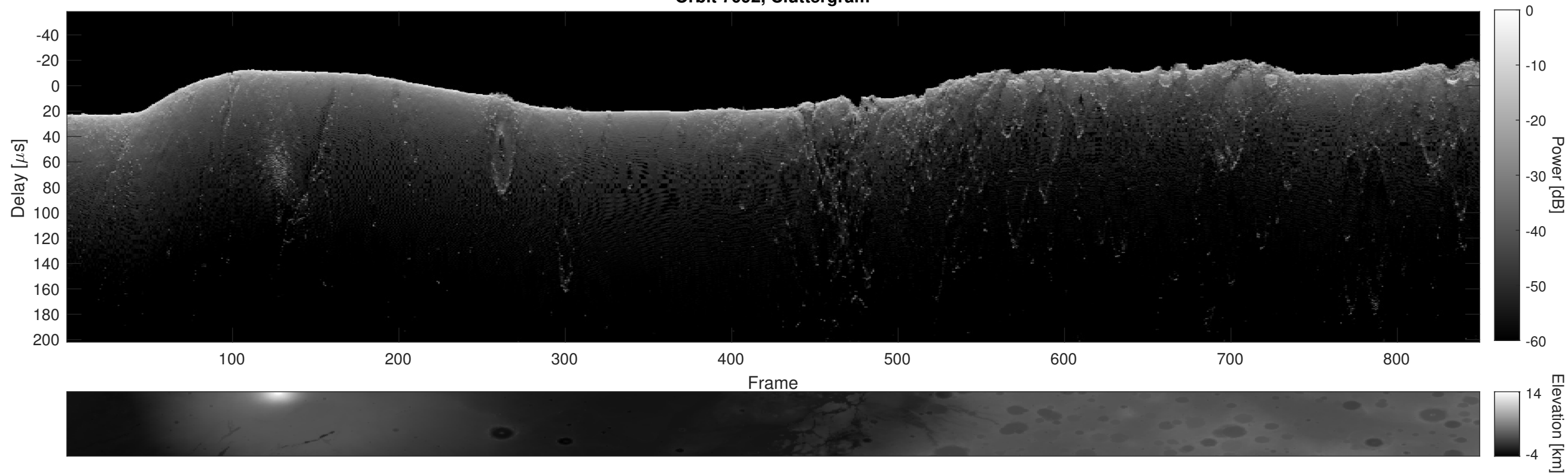
Orbit 7092, Cluttergram
