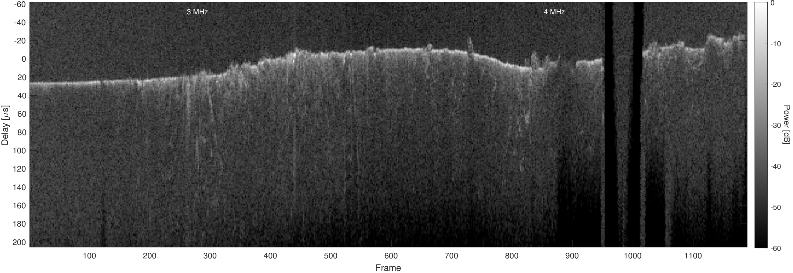
Orbit 7096, Optimized, Window, Channel 2
