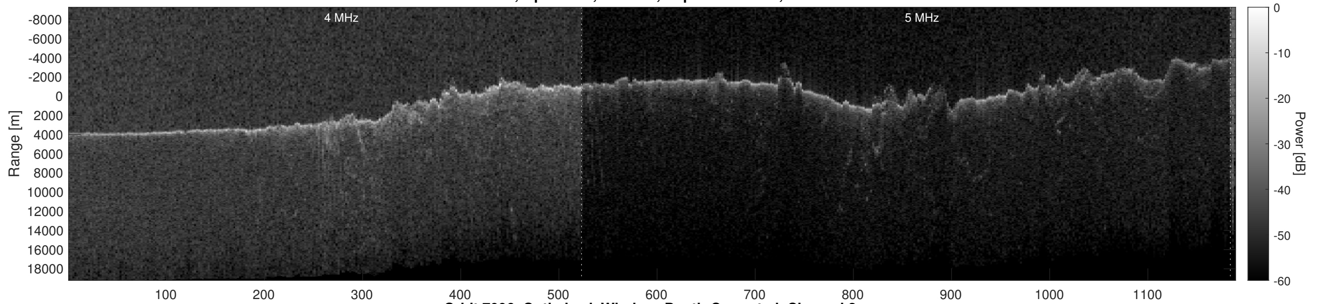
Orbit 7096, Optimized, Window, Depth-Corrected, Channel 2
