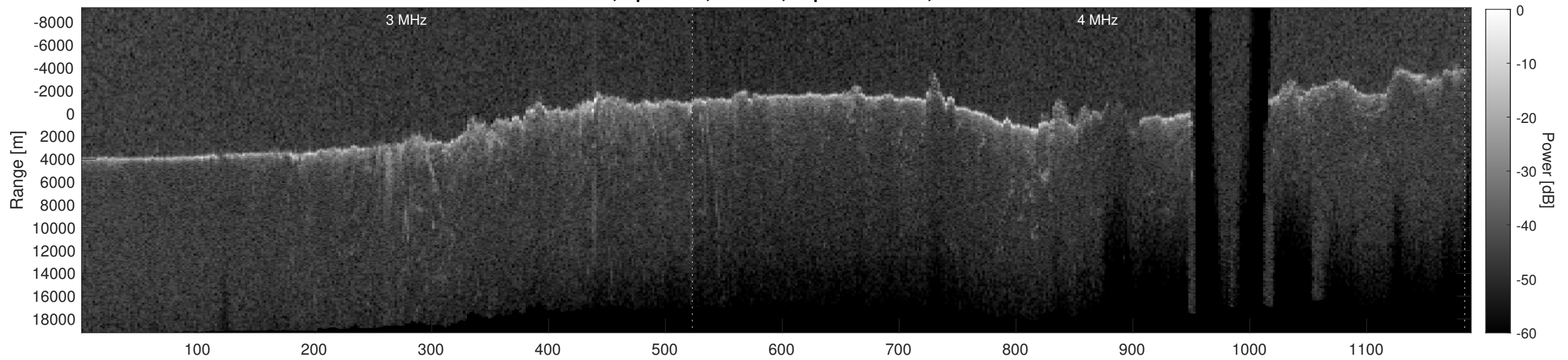
Orbit 7096, Depth-Corrected Cluttergram
