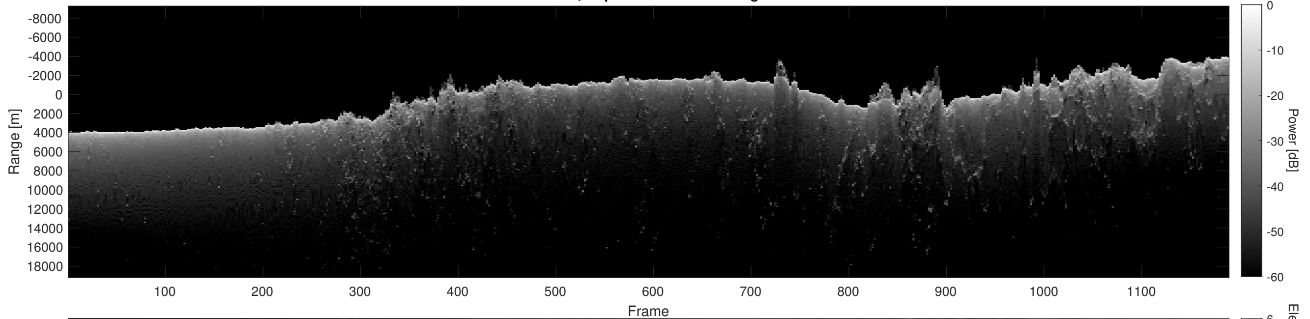
Orbit 7096, Depth-Corrected Cluttergram
