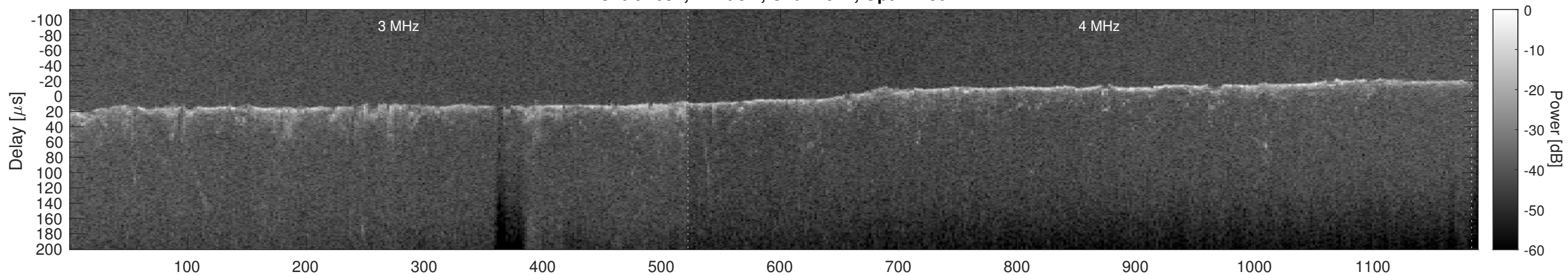
Orbit 7097, Cluttergram
