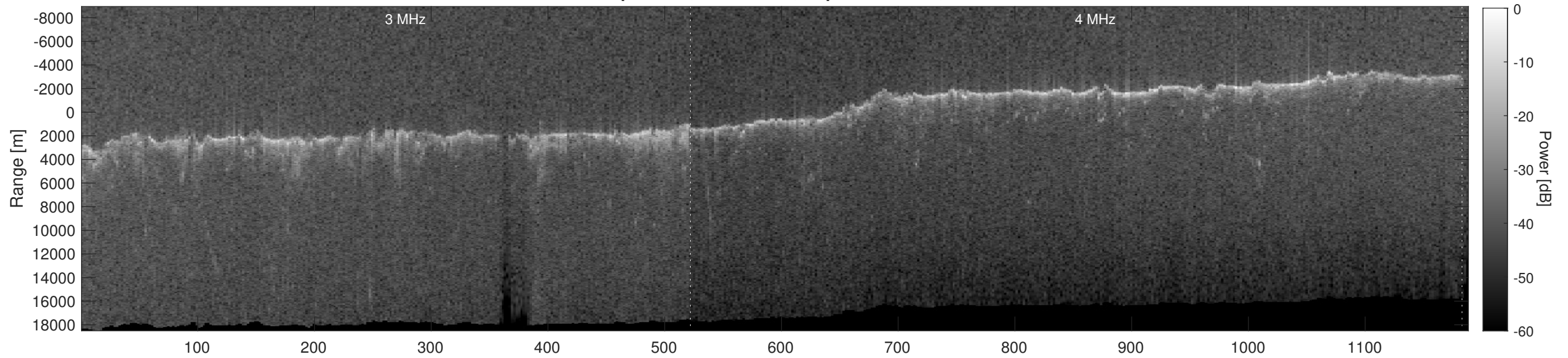
Orbit 7097, Depth-Corrected Cluttergram
