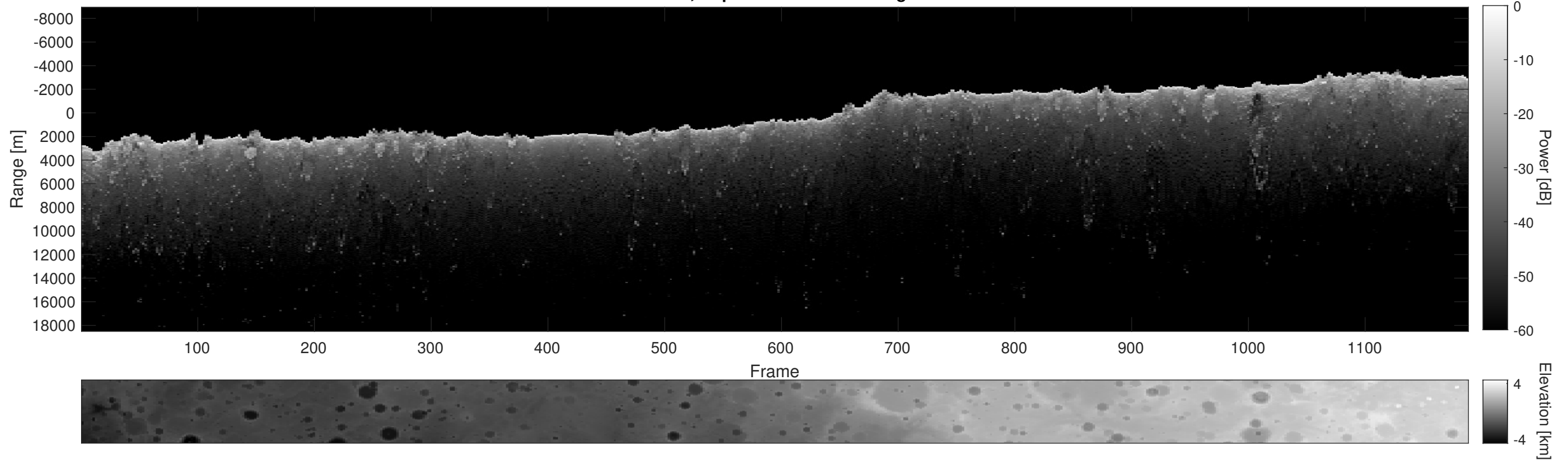
Orbit 7097, Depth-Corrected Cluttergram
