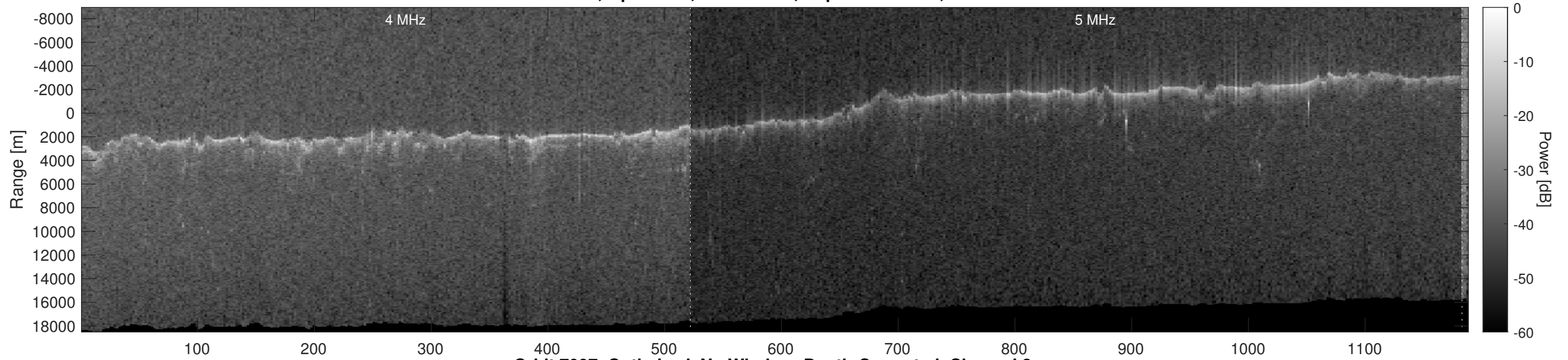
Orbit 7097, Optimized, No Window, Depth-Corrected, Channel 2
