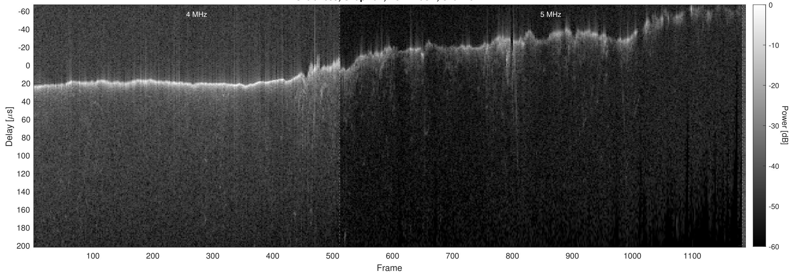
Orbit 7099, Chapman, No Window, Channel 2
