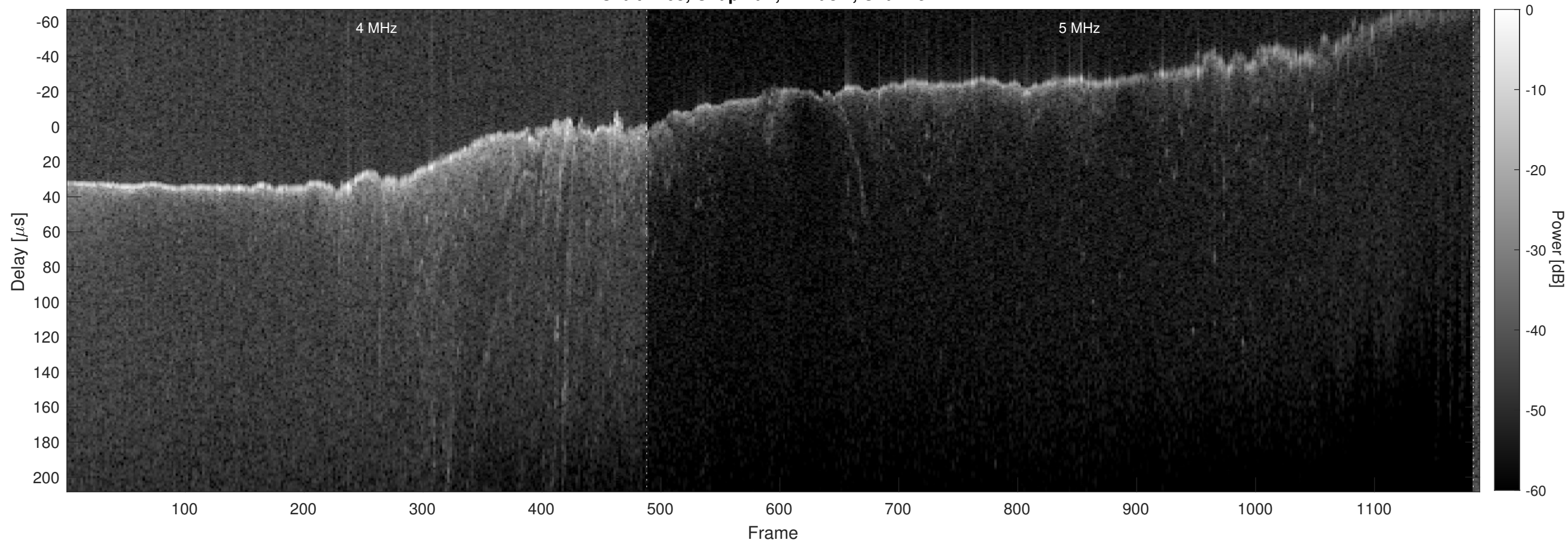
Orbit 7103, Chapman, Window, Channel 2
