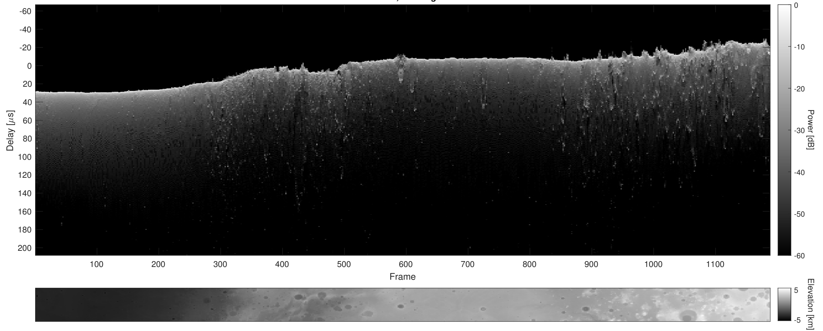
Orbit 7103, Cluttergram
