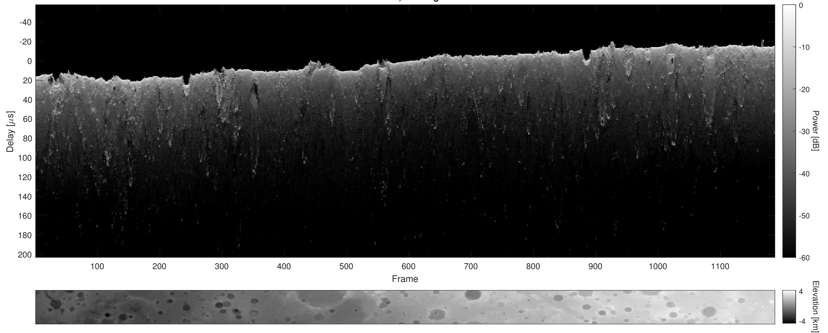
Orbit 7104, Cluttergram
