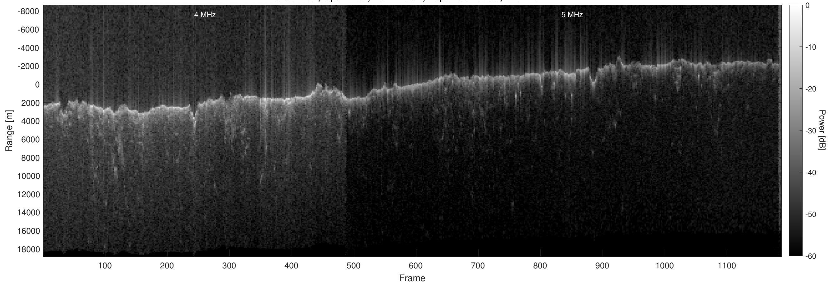
Orbit 7104, Optimized, No Window, Depth-Corrected, Channel 2
