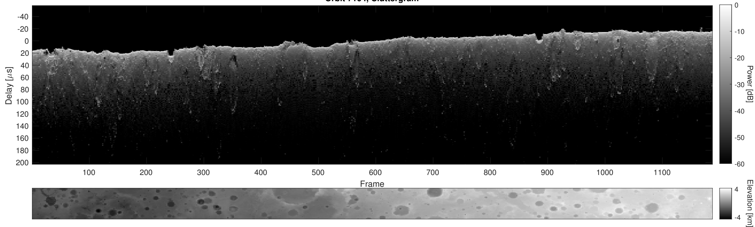
Orbit 7104, Cluttergram
