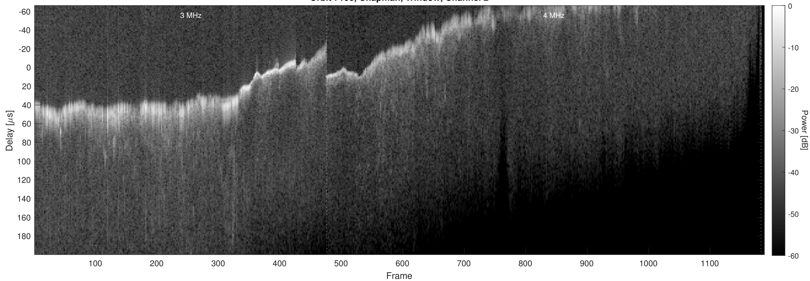
Orbit 7106, Chapman, Window, Channel 2
