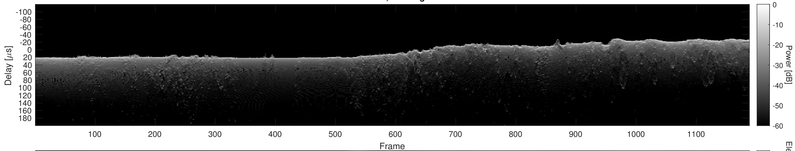
Orbit 7106, Cluttergram
