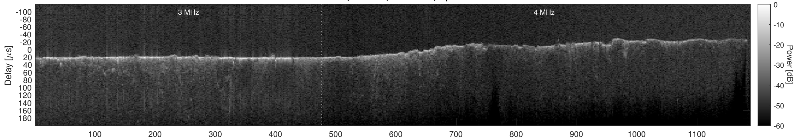
Orbit 7106, Cluttergram
