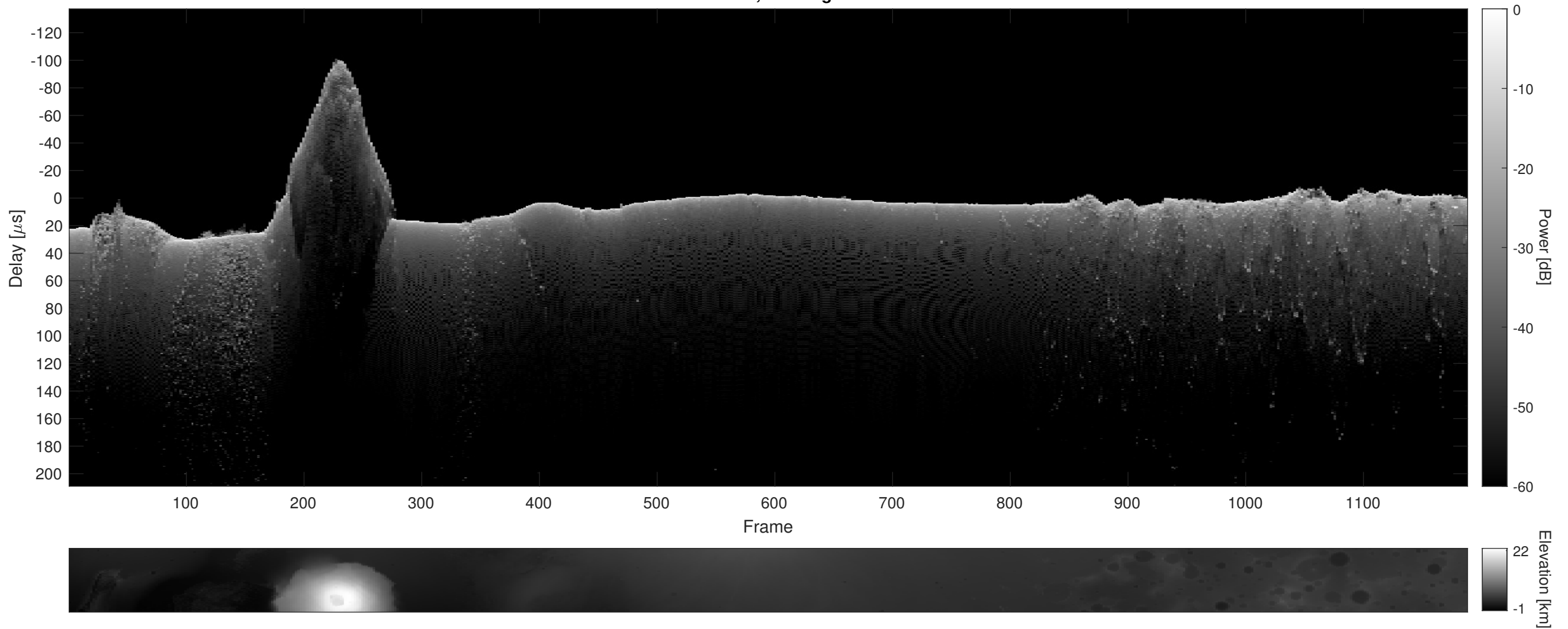
Orbit 7109, Cluttergram
