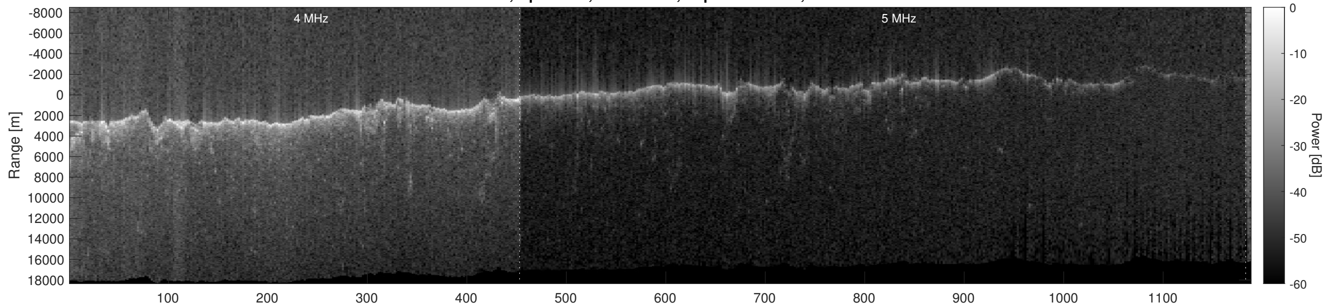
Orbit 7111, Optimized, No Window, Depth-Corrected, Channel 2
