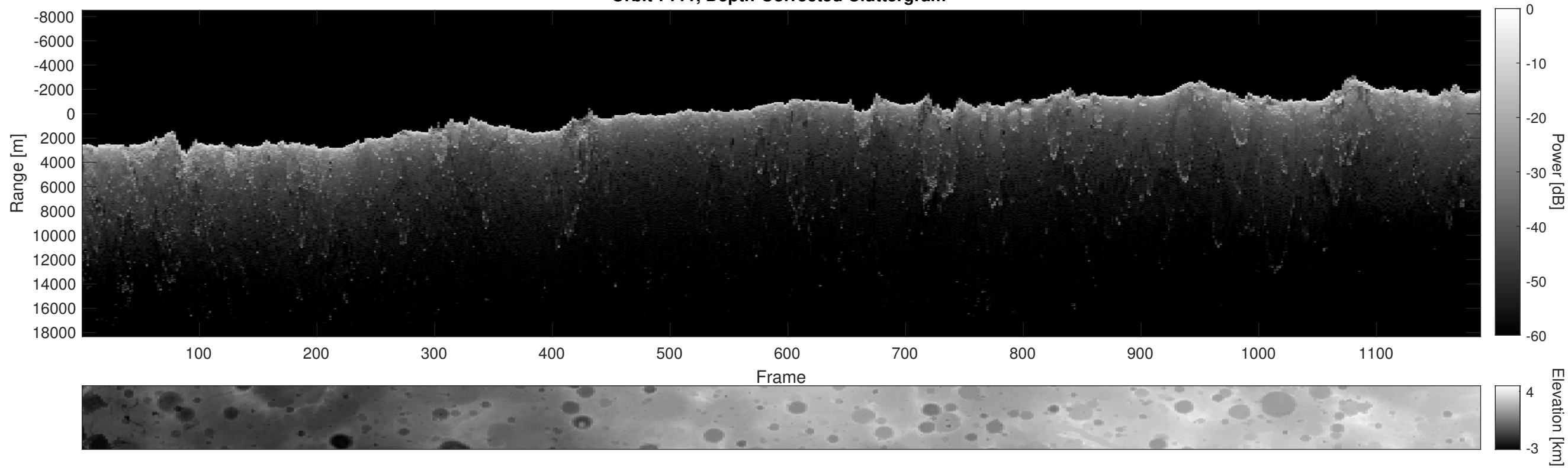
Orbit 7111, Depth-Corrected Cluttergram
