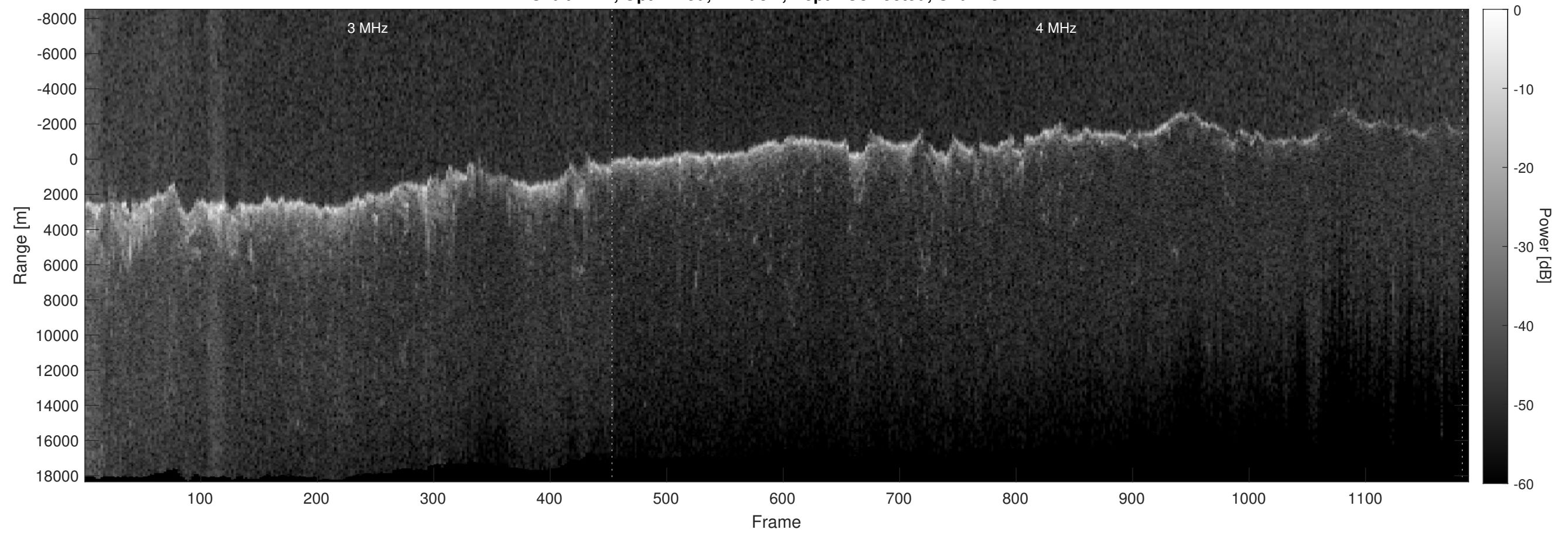
Orbit 7111, Optimized, Window, Depth-Corrected, Channel 2
