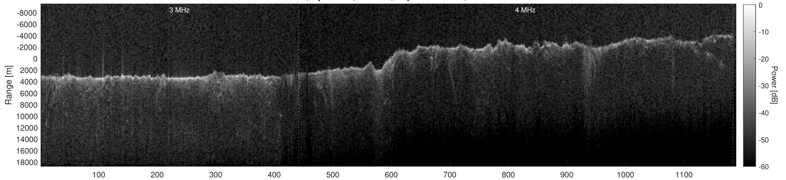
Orbit 7113, Depth-Corrected Cluttergram
