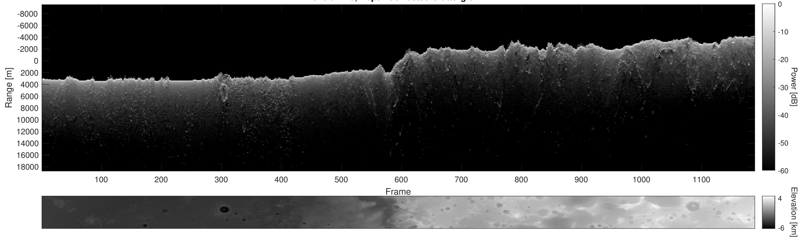
Orbit 7113, Depth-Corrected Cluttergram
