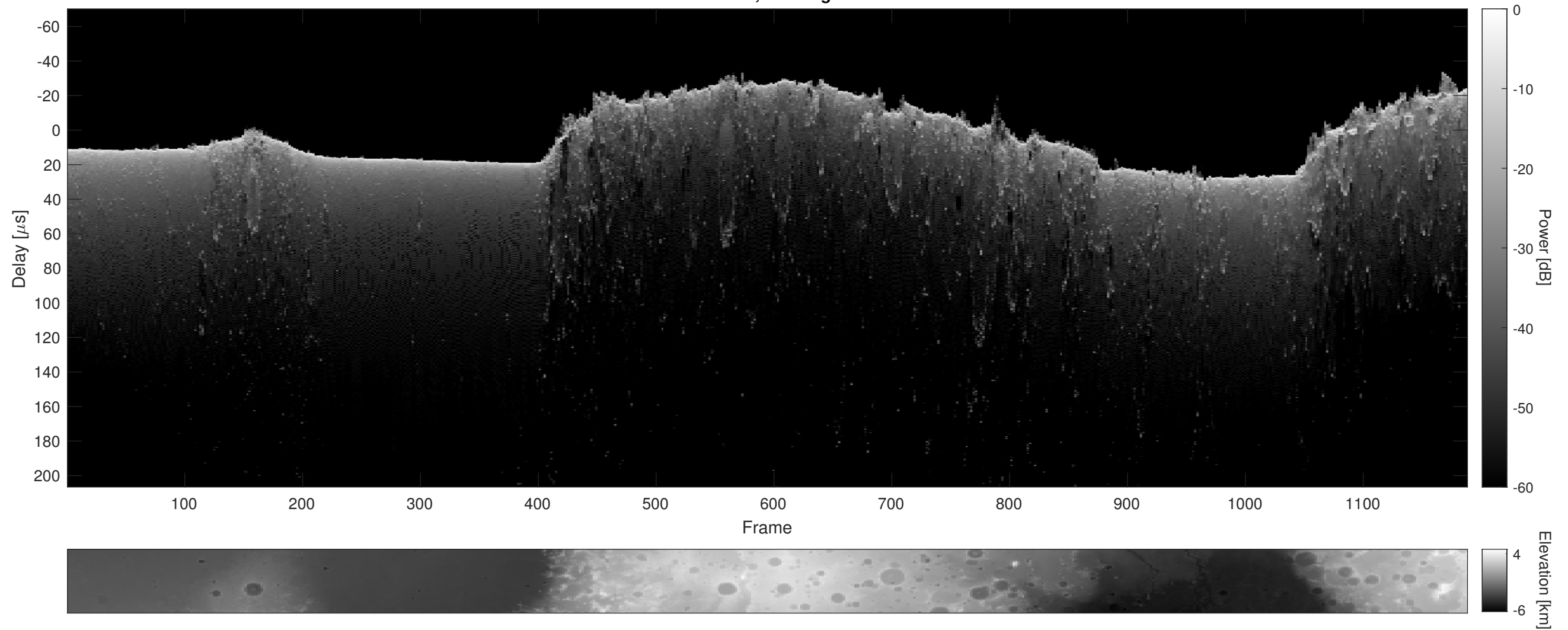
Orbit 7114, Cluttergram
