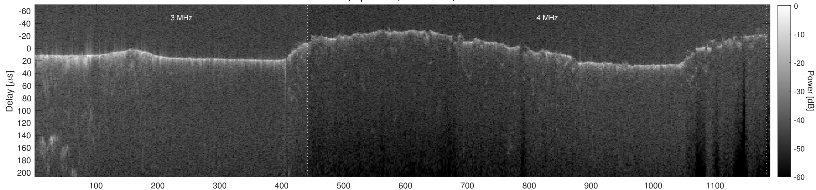
Orbit 7114, Cluttergram
