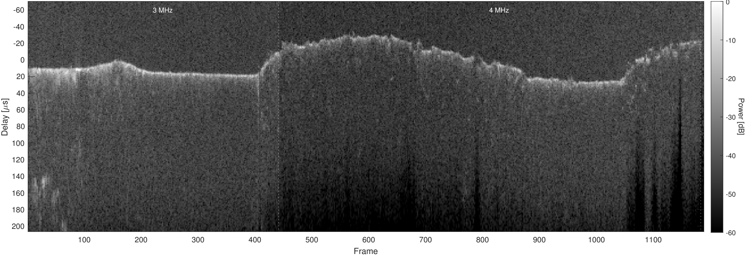
Orbit 7114, Optimized, Window, Channel 2
