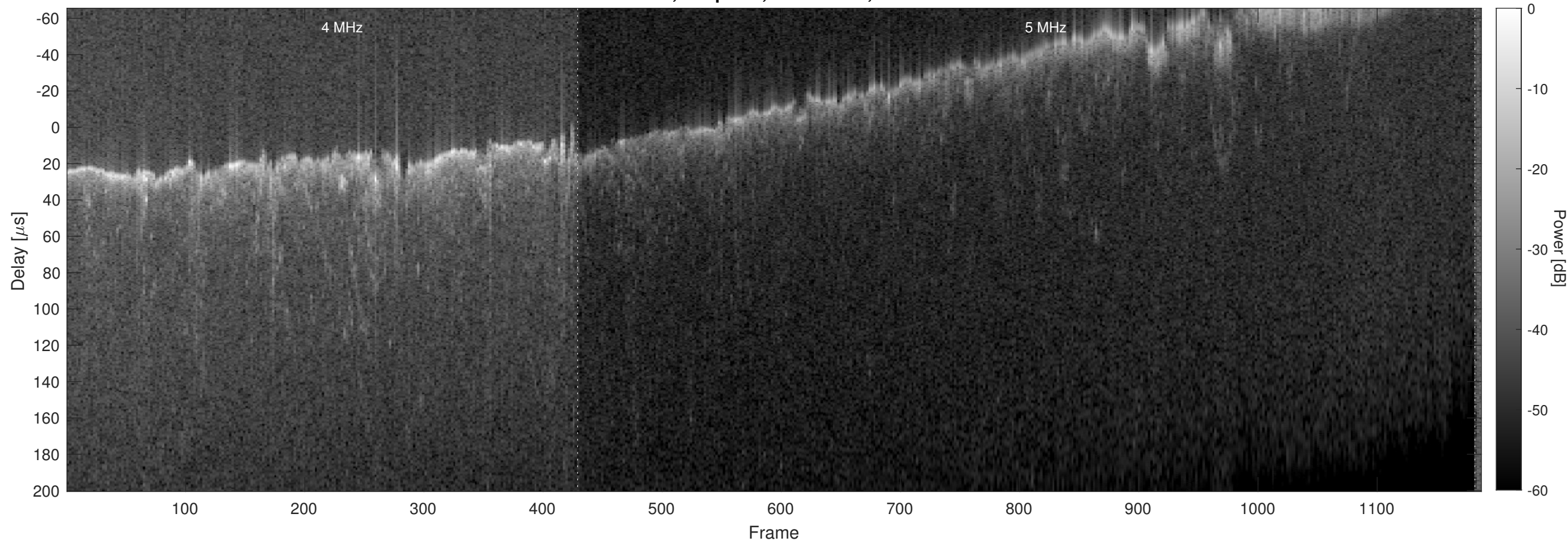
Orbit 7115, Chapman, No Window, Channel 2
