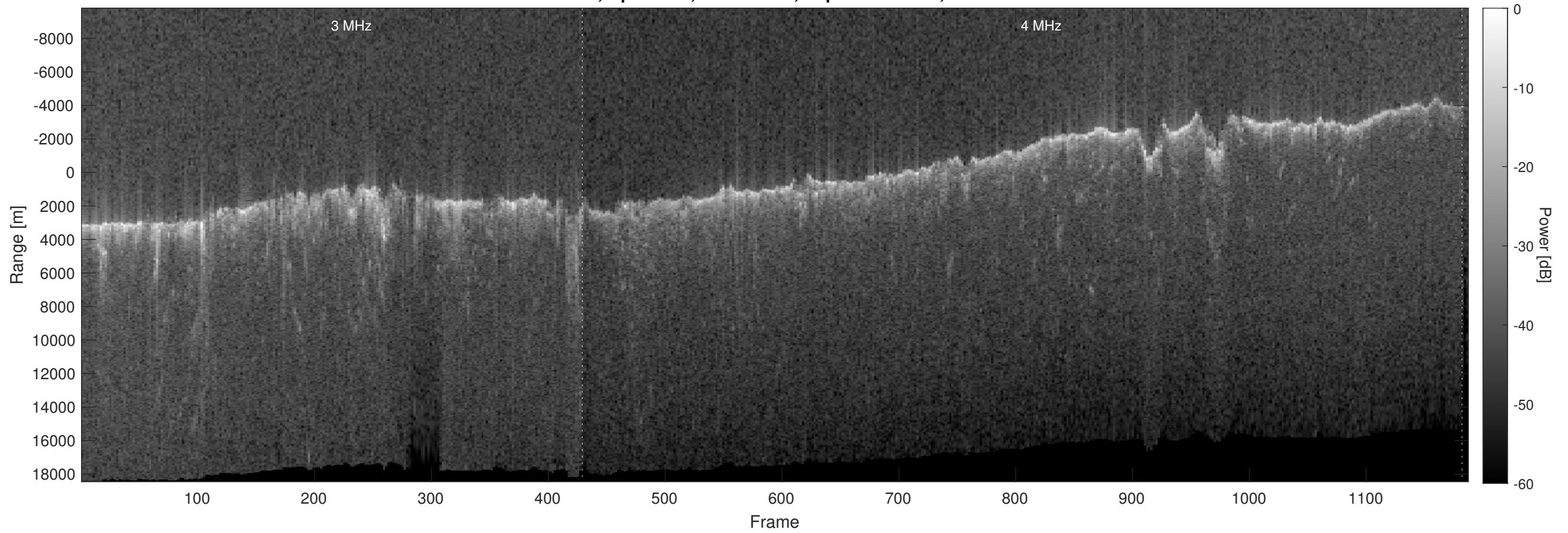
Orbit 7115, Optimized, No Window, Depth-Corrected, Channel 2
