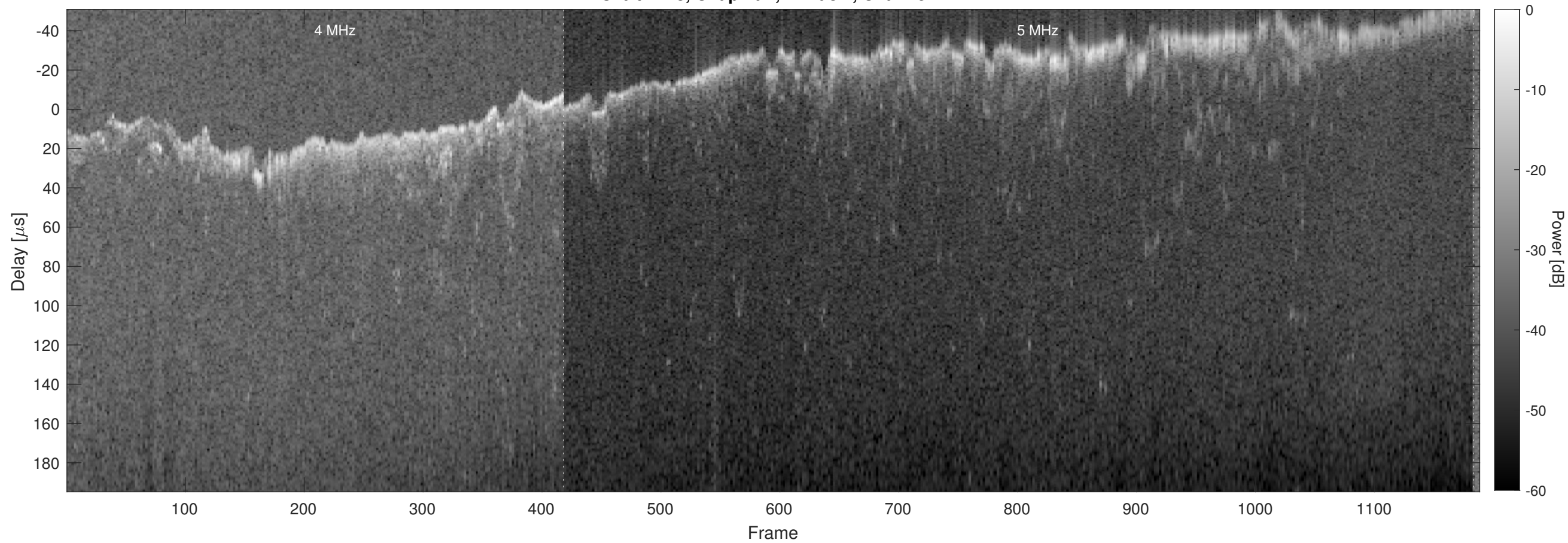
Orbit 7118, Chapman, Window, Channel 2
