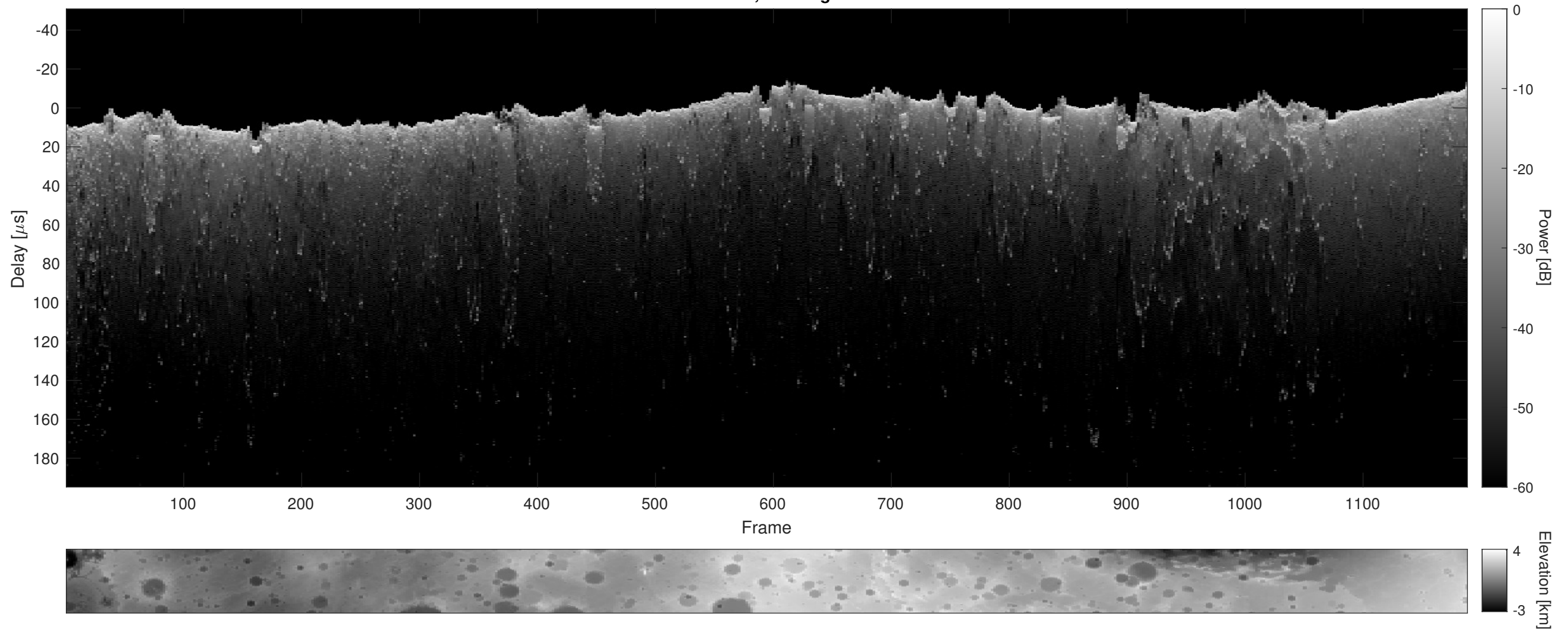
Orbit 7118, Cluttergram
