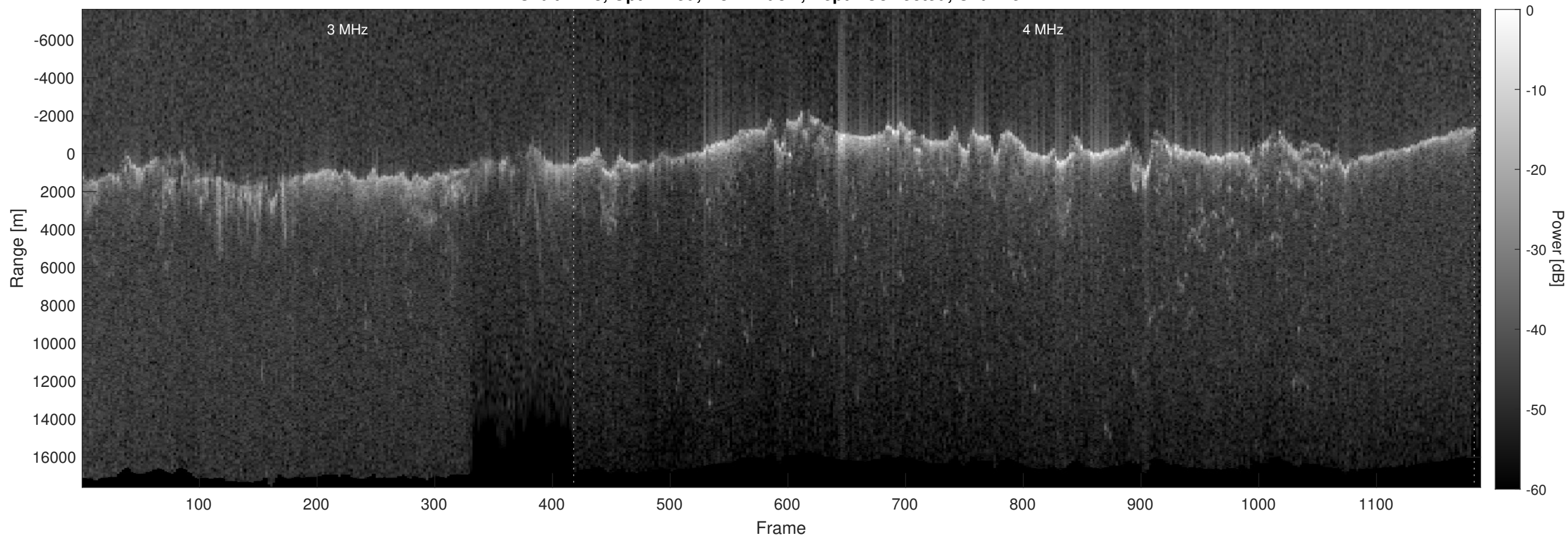
Orbit 7118, Optimized, No Window, Depth-Corrected, Channel 2
