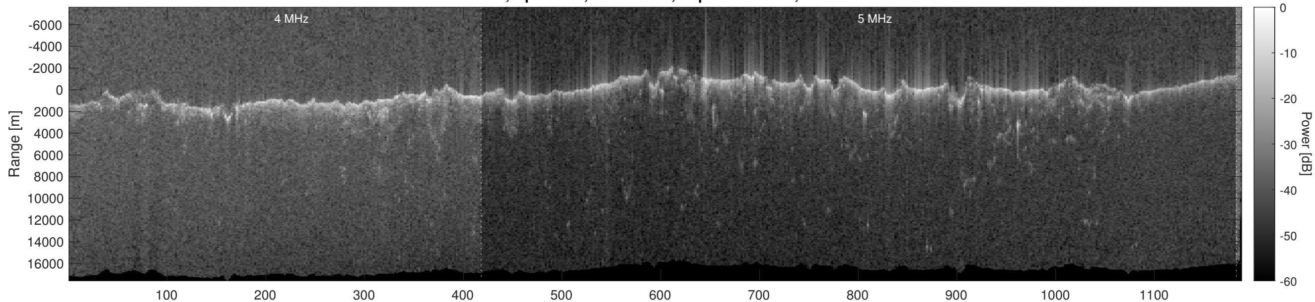
Orbit 7118, Optimized, No Window, Depth-Corrected, Channel 2
