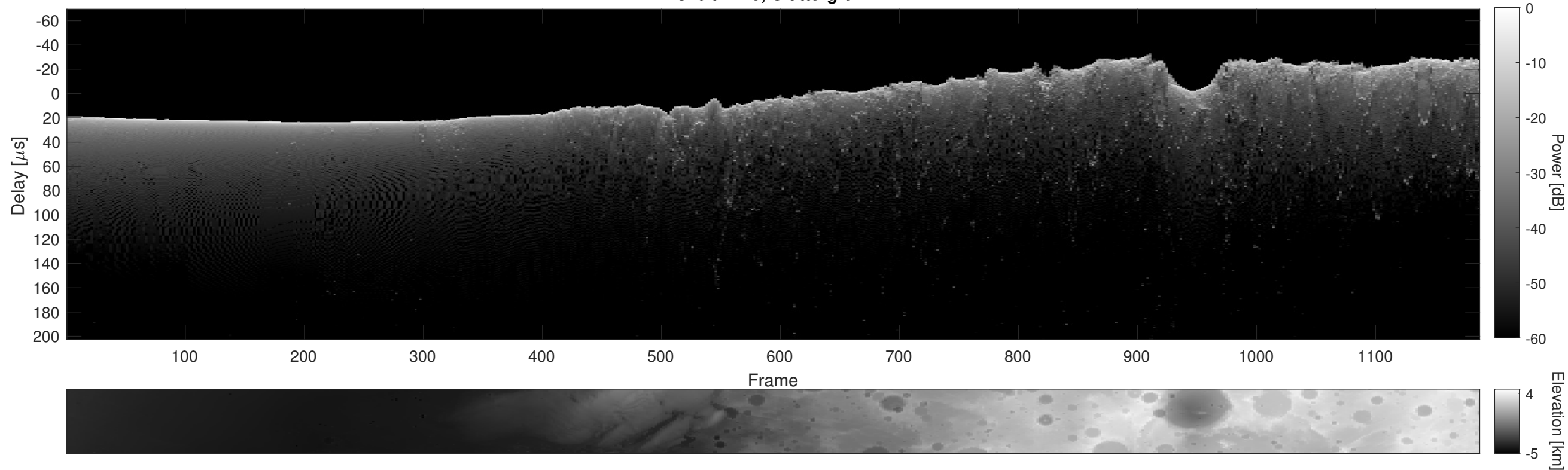
Orbit 7120, Cluttergram
