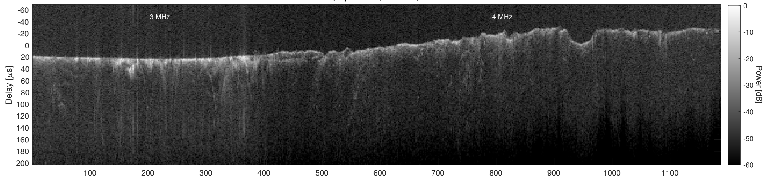
Orbit 7120, Cluttergram
