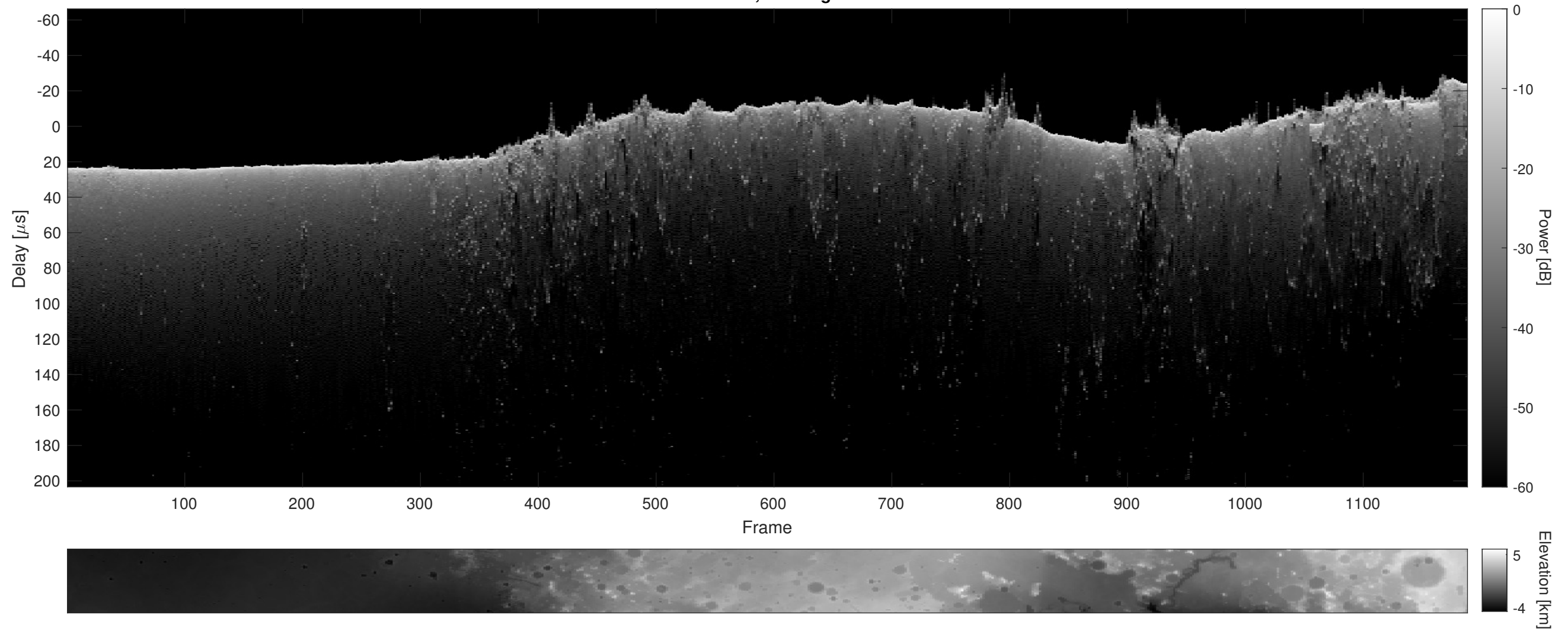
Orbit 7121, Cluttergram
