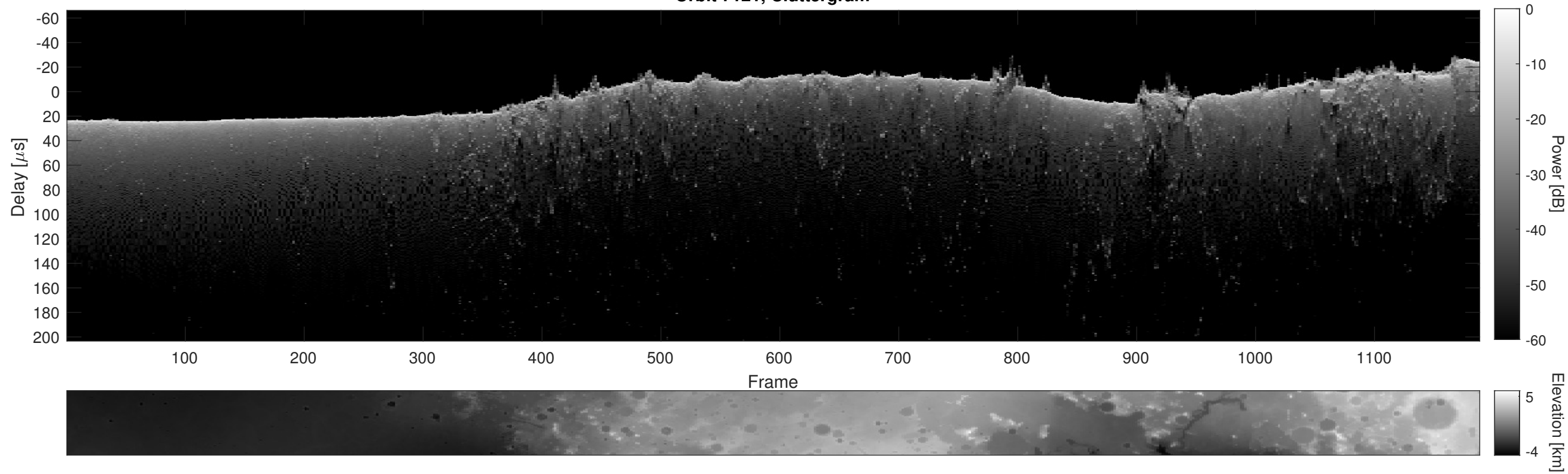
Orbit 7121, Cluttergram
