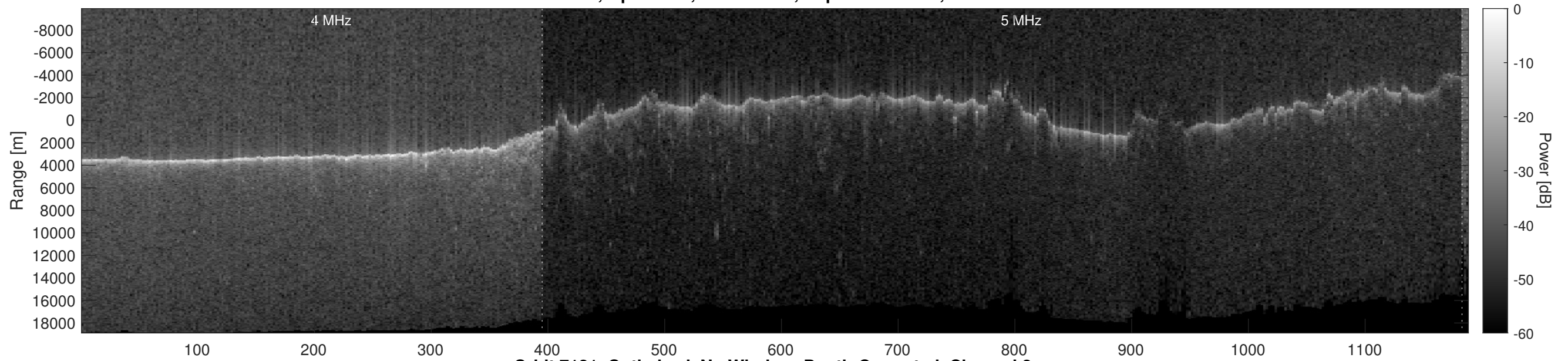
Orbit 7121, Optimized, No Window, Depth-Corrected, Channel 2
