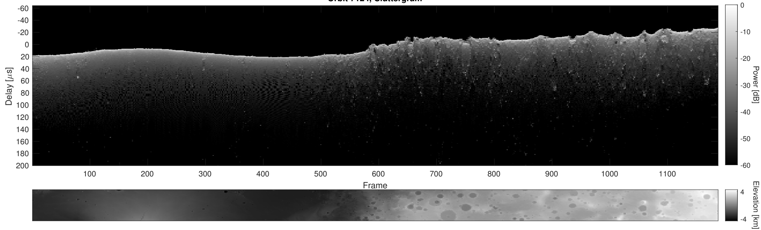
Orbit 7124, Cluttergram
