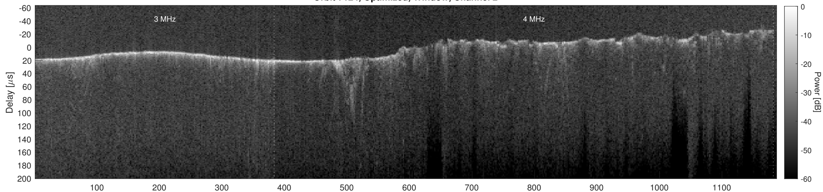
Orbit 7124, Cluttergram
