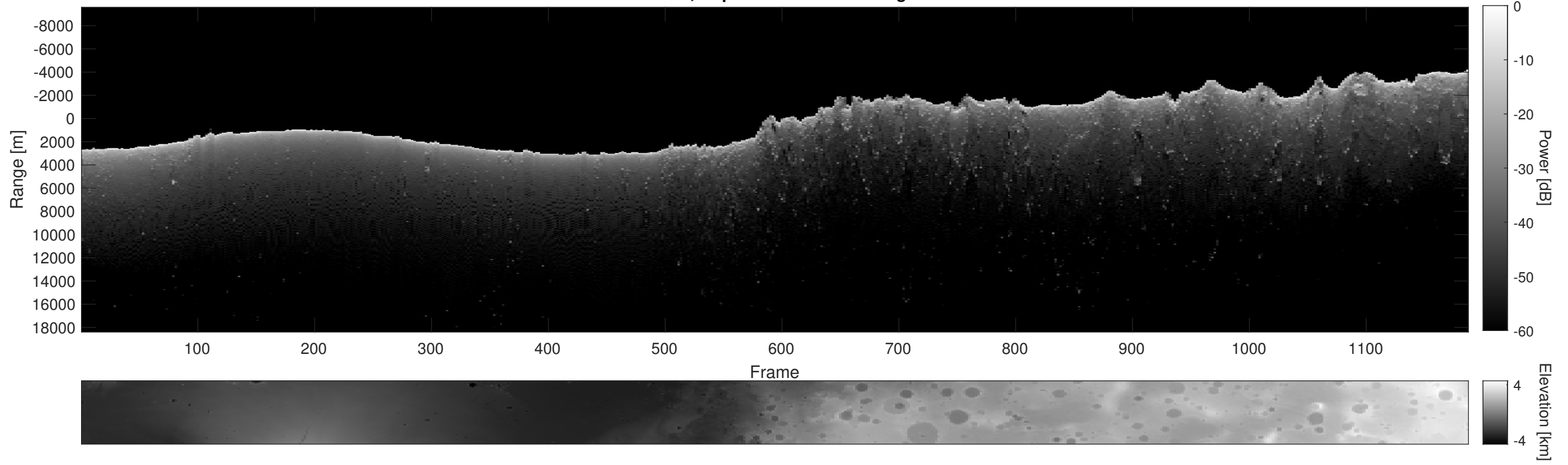
Orbit 7124, Depth-Corrected Cluttergram
