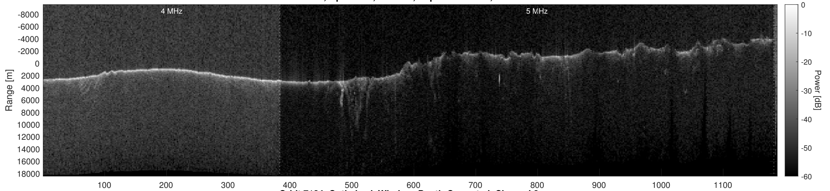
Orbit 7124, Optimized, Window, Depth-Corrected, Channel 2
