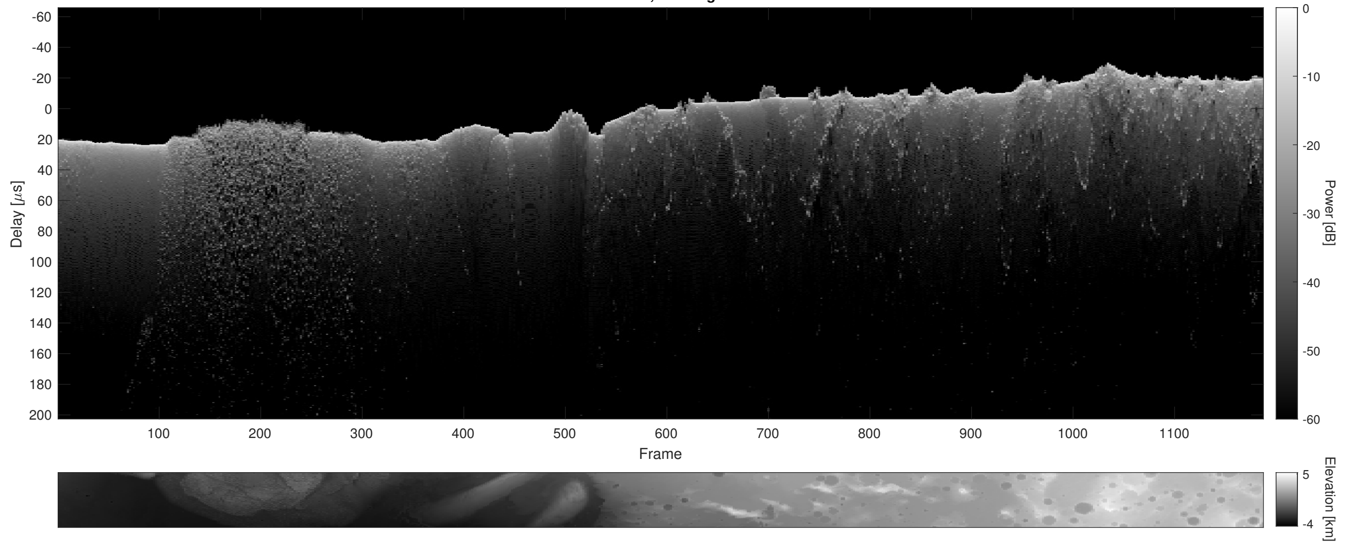
Orbit 7127, Cluttergram
