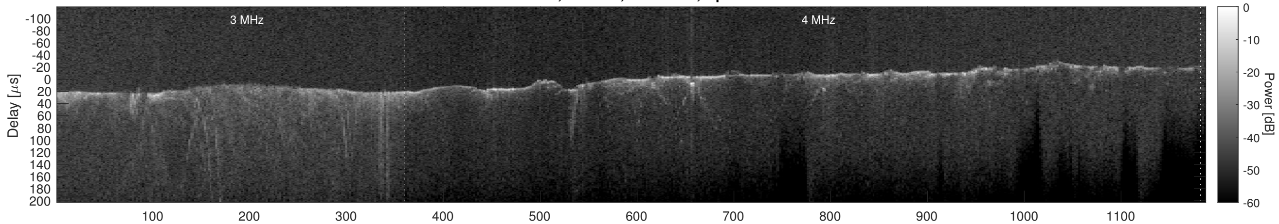
Orbit 7127, Cluttergram
