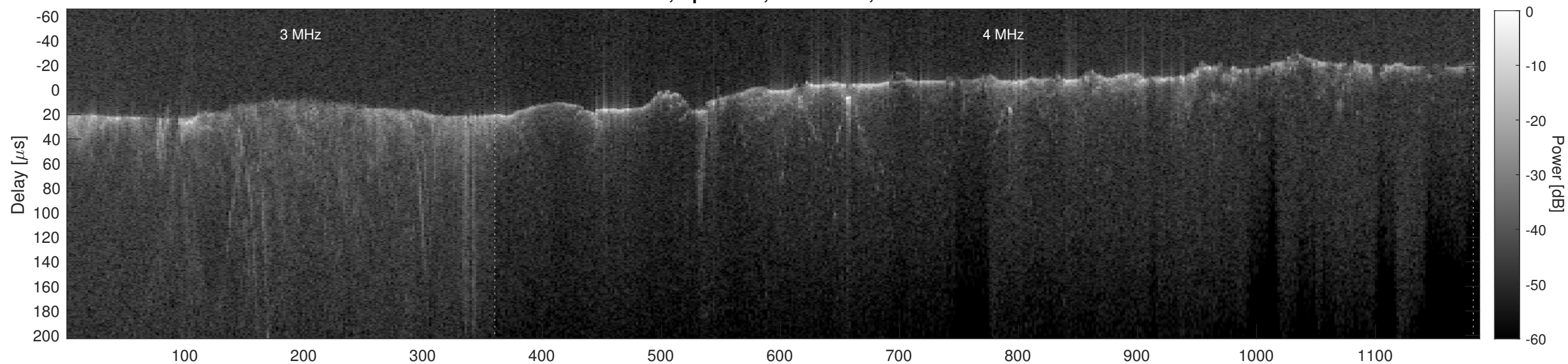
Orbit 7127, Cluttergram
