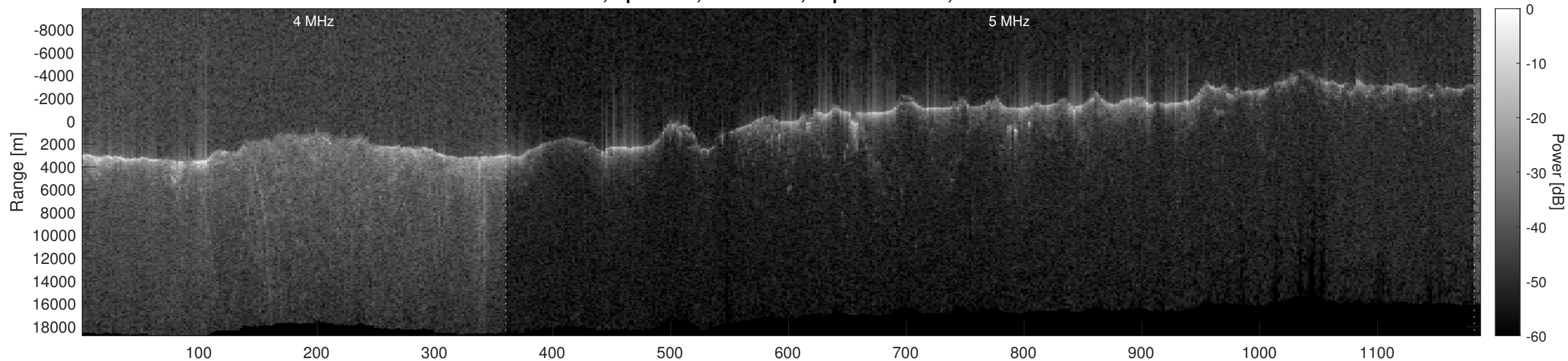
Orbit 7127, Optimized, No Window, Depth-Corrected, Channel 2
