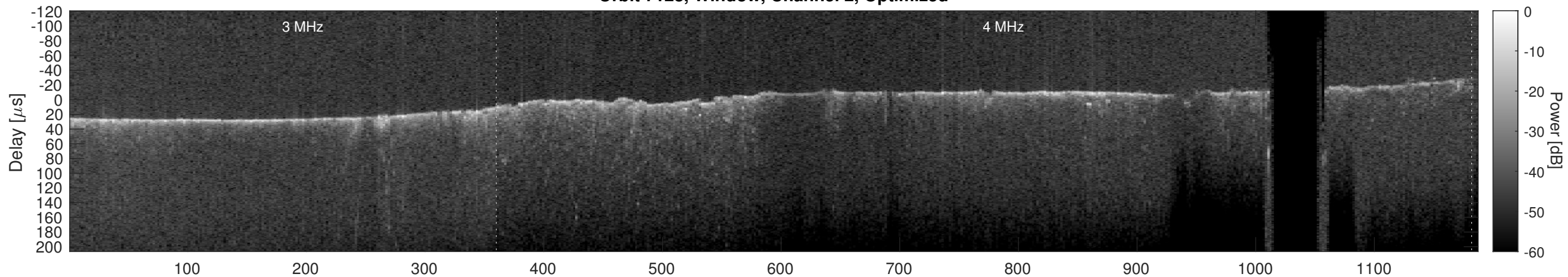
Orbit 7128, Cluttergram
