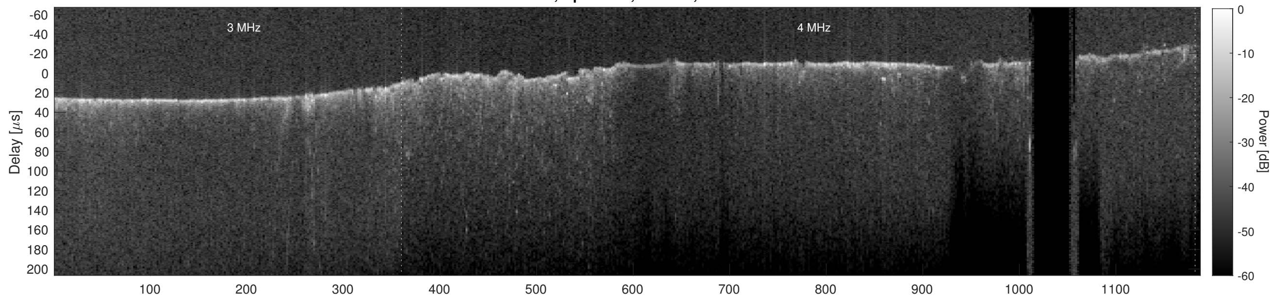
Orbit 7128, Cluttergram
