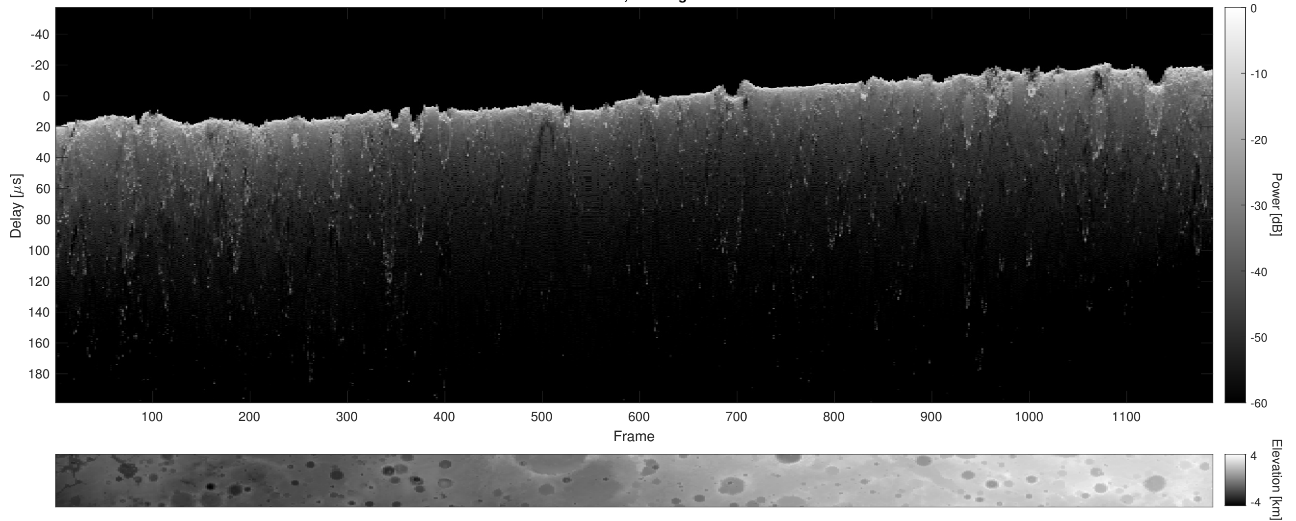
Orbit 7129, Cluttergram
