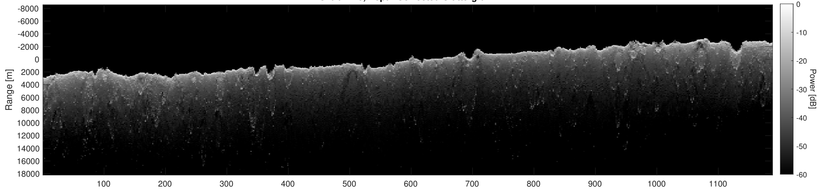
Orbit 7129, Depth-Corrected Cluttergram
