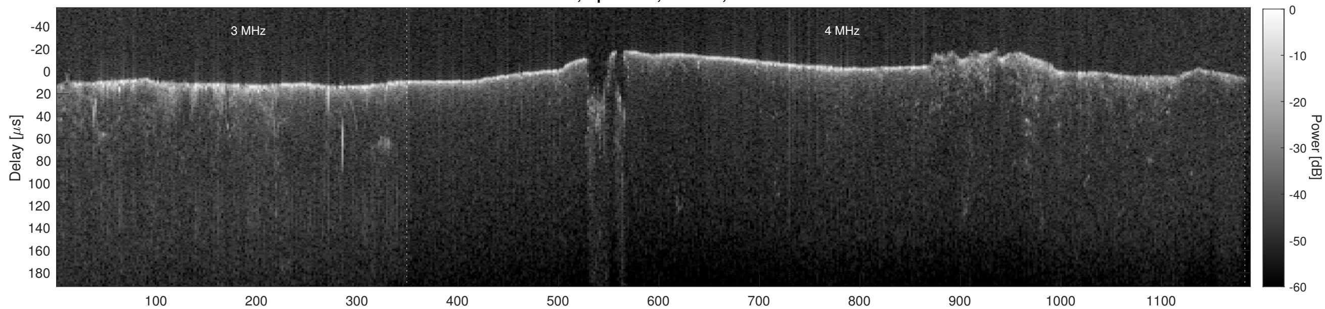
Orbit 7130, Cluttergram
