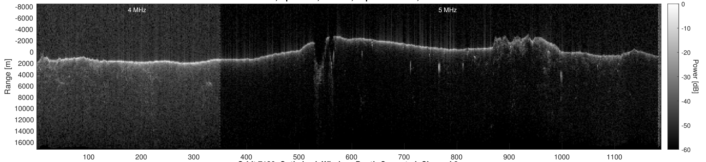
Orbit 7130, Optimized, Window, Depth-Corrected, Channel 2
