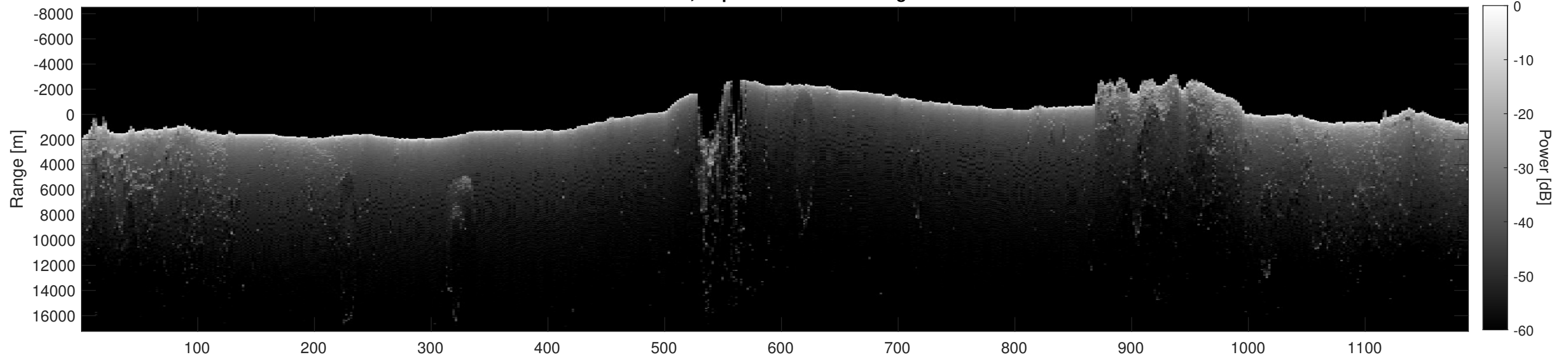
Orbit 7130, Depth-Corrected Cluttergram
