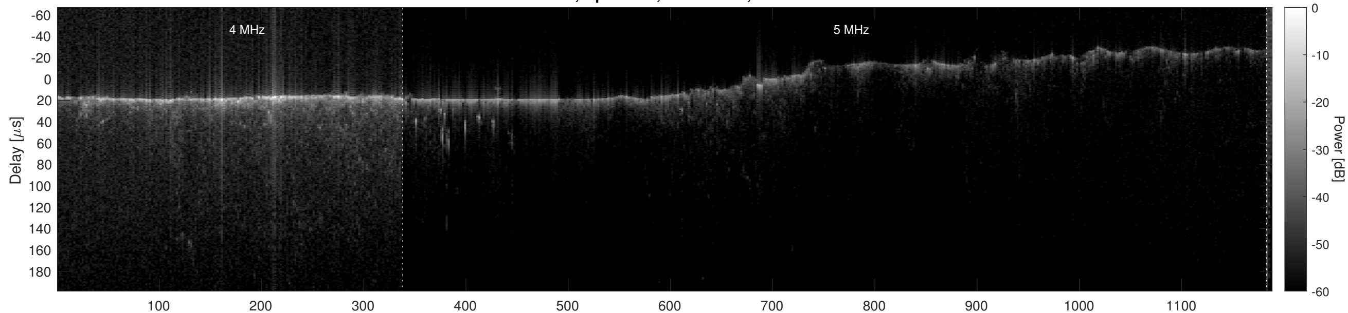
Orbit 7131, Optimized, No Window, Channel 2
