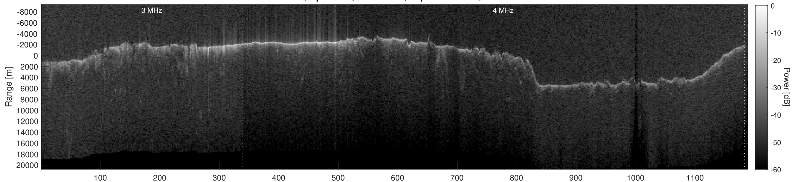
Orbit 7132, Depth-Corrected Cluttergram
