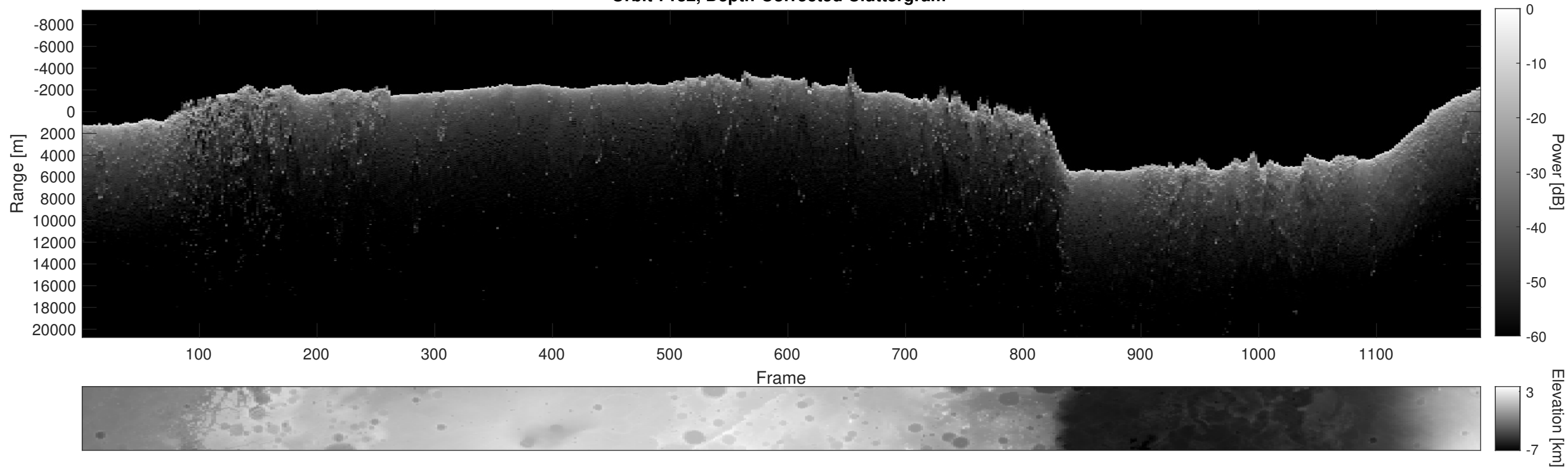
Orbit 7132, Depth-Corrected Cluttergram
