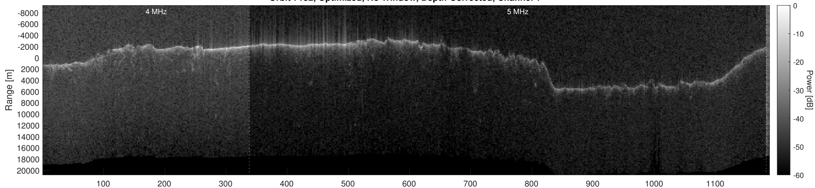
Orbit 7132, Optimized, No Window, Depth-Corrected, Channel 2
