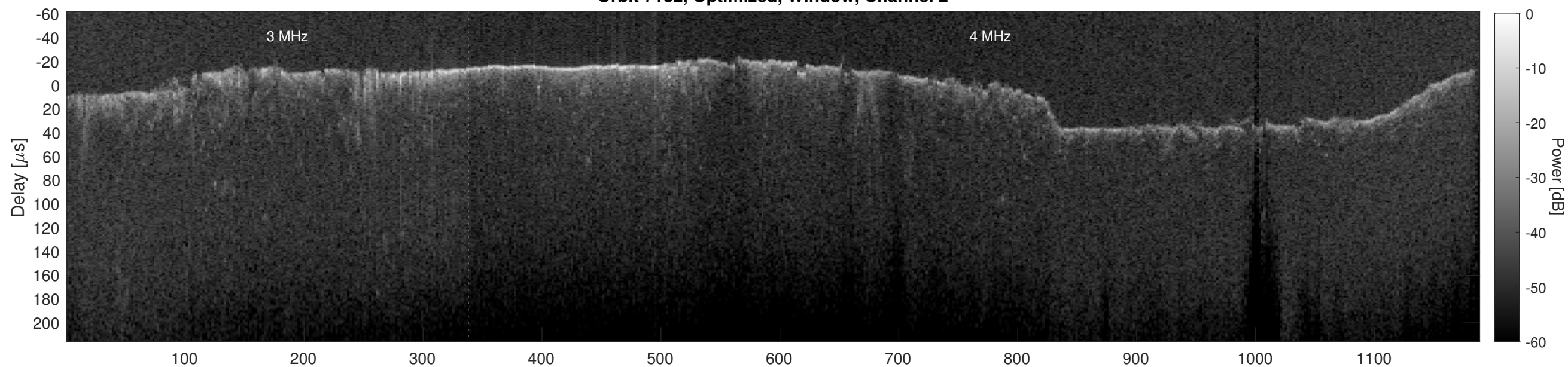
Orbit 7132, Cluttergram
