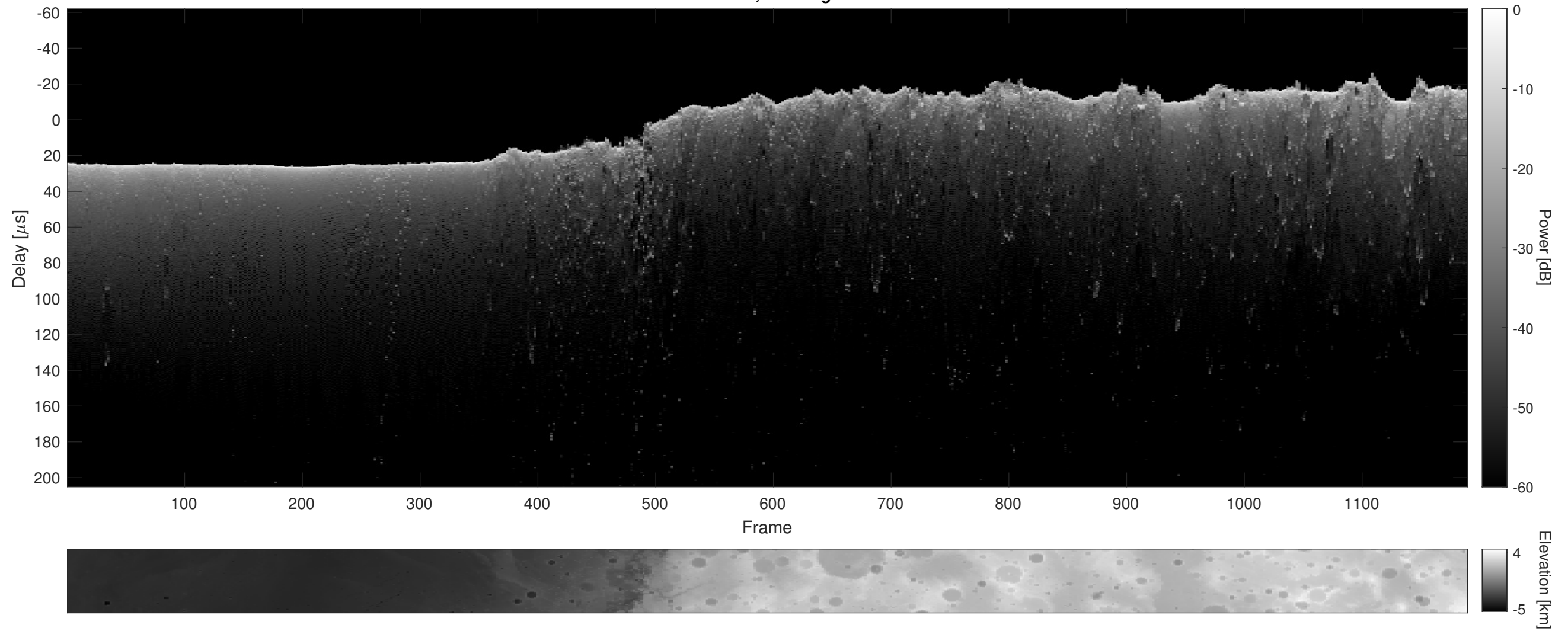
Orbit 7135, Cluttergram
