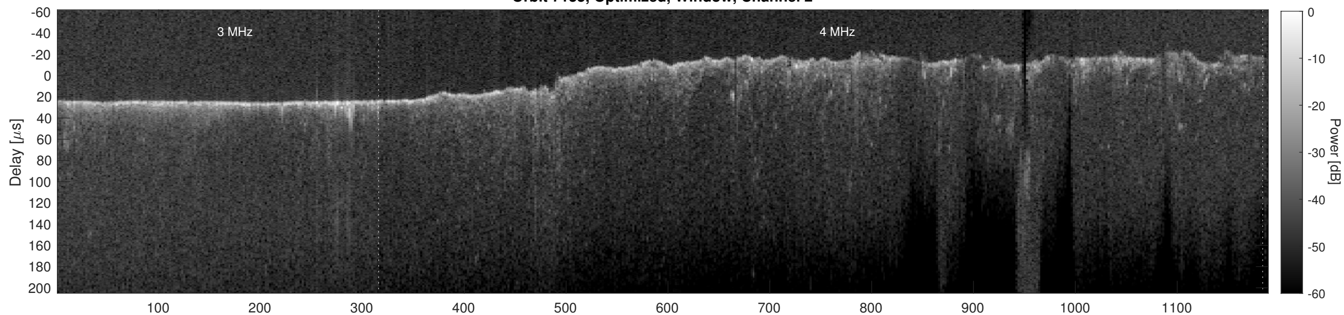
Orbit 7135, Cluttergram
