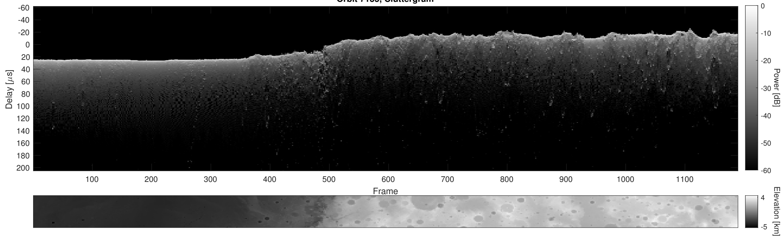
Orbit 7135, Cluttergram
