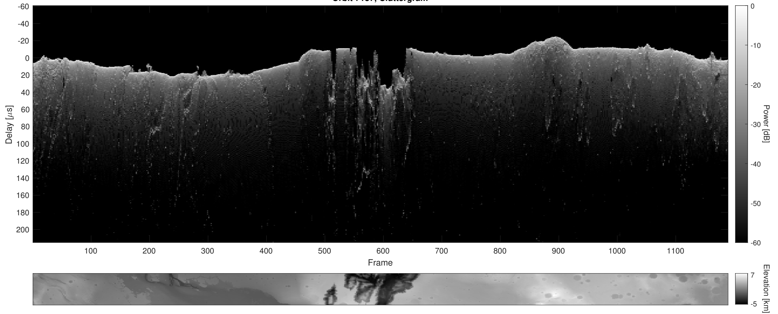
Orbit 7137, Cluttergram
