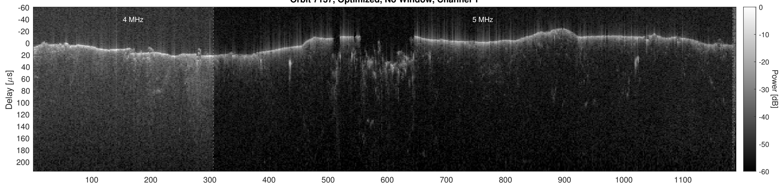
Orbit 7137, Optimized, No Window, Channel 2
